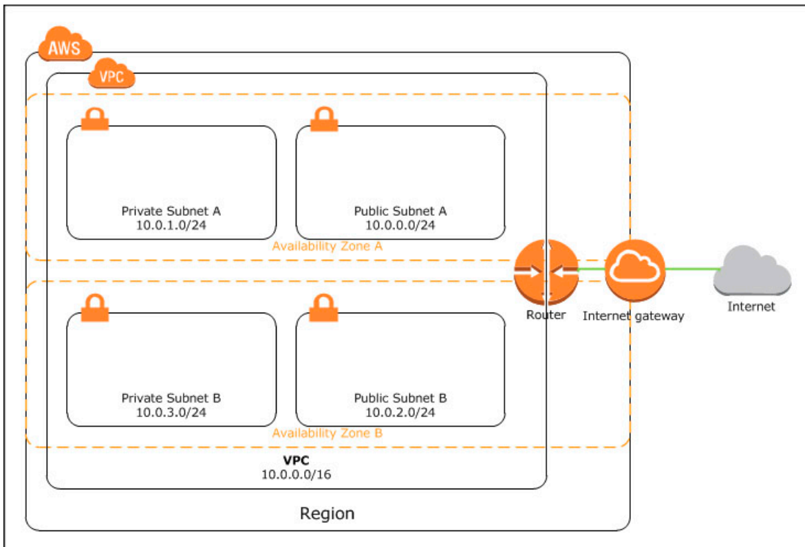
Multi-AZ VPC
