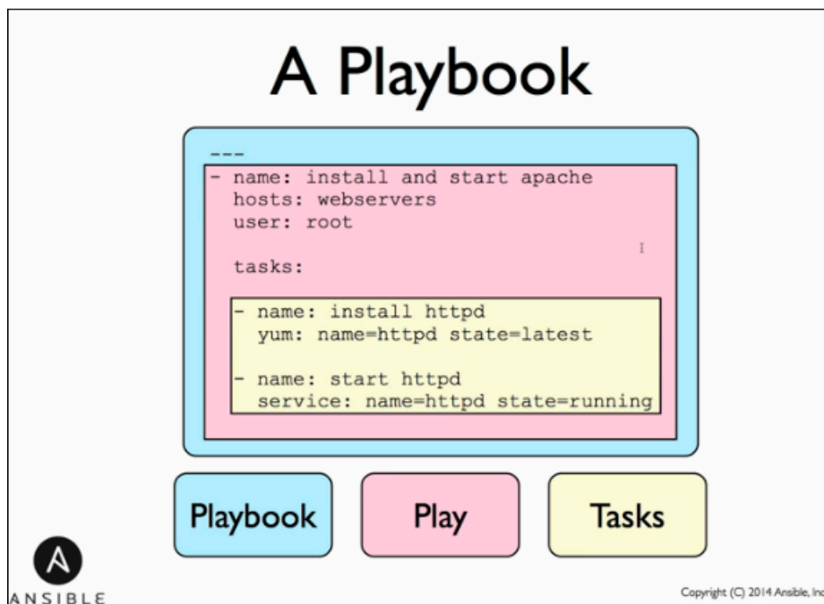
Ansible Playbook
