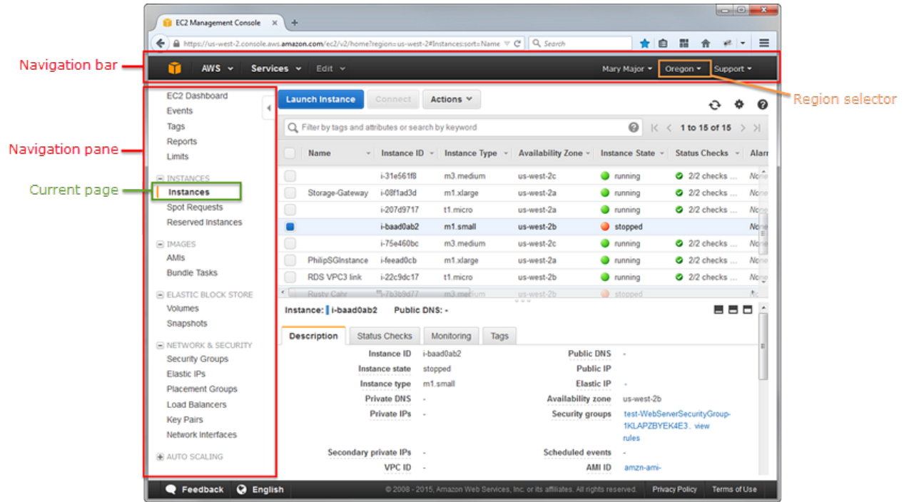
EC2 Console
